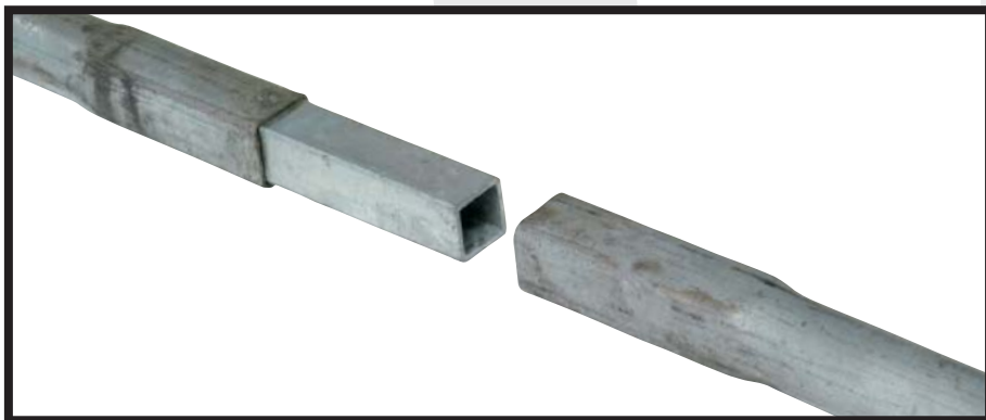
Galvanized tube conical end with square junction
