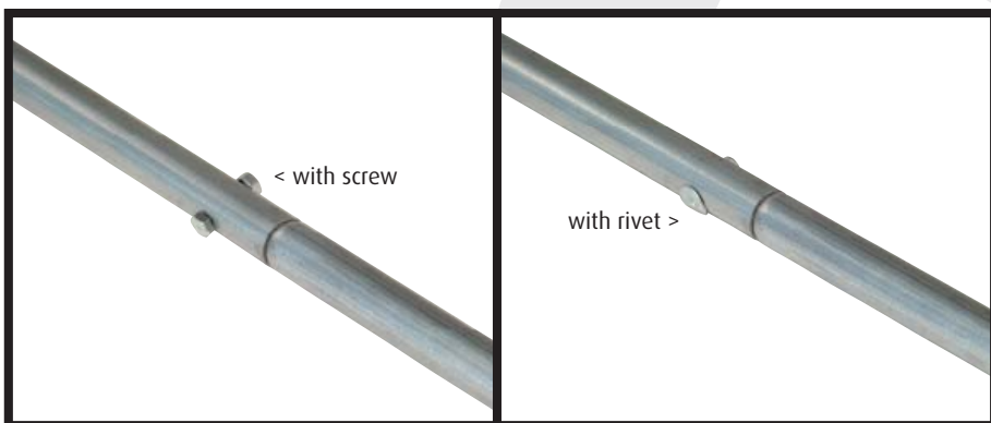
Galvanized tube with conical end \varnothing 28-32 mm. two versions
